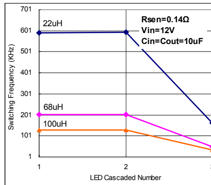
I_{OUT}=700mA
