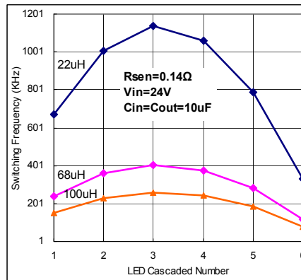
I_{OUT}=700mA
