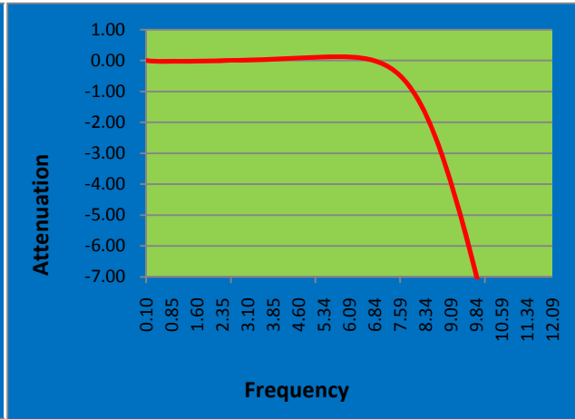
Figure 4. SD Flatness
